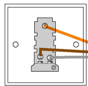
Ei159 Locator Switch
