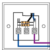
MCP400 Manual Call Point
