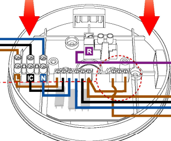
Ei128R Relay Pattress
